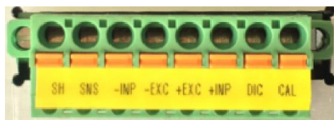
Phoenix Connector-8 pins
